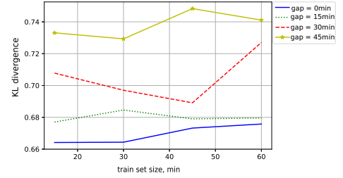
Fig. 5. KL divergence for BISN as a function of the length of the training data [min], and for different gaps between the training and test period.
