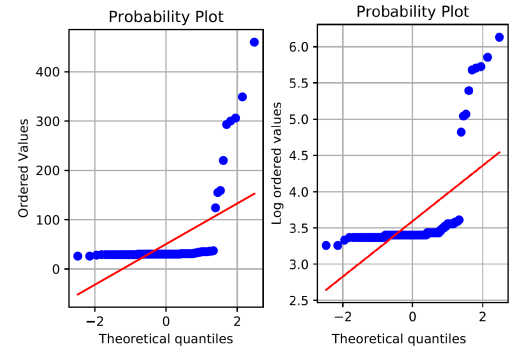
Fig. 3. QQ (quantile-quantile) plots of travel times and log travel times for the most traversed trajectory during one time interval.
